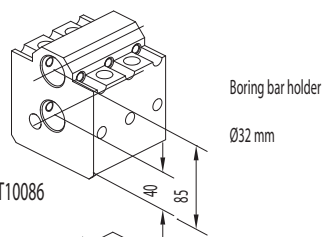
KMS-T13064 (Ø40 mm) 128-22540 (Ø50 mm) Combi toolholder for boring bar and insertdrill with internal coolant
