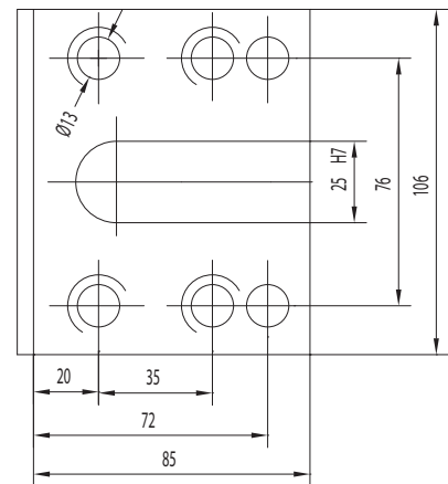
Cut-off tool 25x25mm
