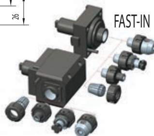
124-06001 124-06003 i.Coolant
