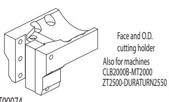
B27008 B27007 Direct mounting on turret
