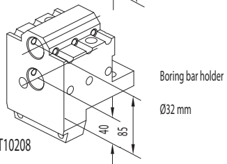
KMS-T10086 Boring bar holder Ø32 mm
