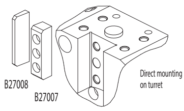
KMS-T00074 Face and O.D. cutting holder Also for machines CLB2000B-MT2000 ZT2500-DURATURN2550
