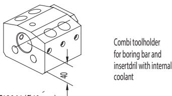
KMS-T10036 (Ø40 mm) KMS-T10044 (Ø50 mm) Boring bar holder
