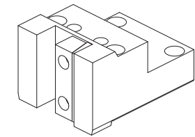
Face and O.D. cutting holder
