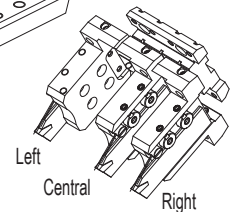
Protection cover 137-00272
